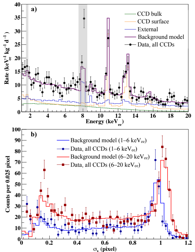
FIG. 2. Projections in E and \sigma_x of the best-fit background model (solid lines) compared to the data (markers). a) The total background model spectrum is shown along with individual contributions from different background sources. Shaded energy regions are excluded from the analysis. b) Comparison of \sigma_x distributions in the fit energy region (red) and extrapolated toward lower energies (blue). The peak at low (high) \sigma_x corresponds to events at the front (back) of the CCDs.
