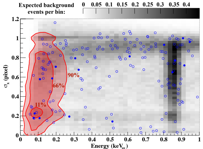
FIG. 3. Best-fit to the final data sample in (E, \sigma_x) space. The blue data points are overlaid on the best-fit background model in gray. Open circles correspond to CCDs 2–7, while filled circles correspond to CCD 1. The red contours represent the best-fit exponential excess with \epsilon=66 eV ee . The Ne K de-excitation line (0.85 keV ee ) emitted following electron capture by 22 Na in the CCD bulk is visible.
