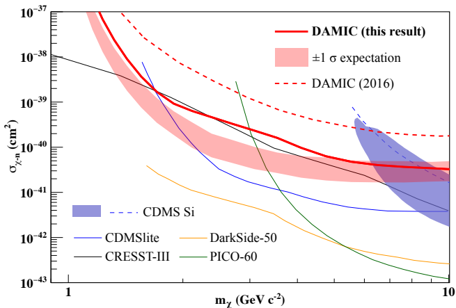
FIG. 4. Upper limit (90% CL) on \sigma_{\chi-n} obtained from this analysis (solid red line). The expectation \pm 1\sigma band if only known backgrounds are present in our data set is shown by the red band. For comparison, we also include 90% CL exclusion limits from our previous result with a 0.6 kg d exposure [11], other experiments [4, 6], and the 90% CL contours for the WIMP-signal interpretation of the CDMS silicon result [4].
